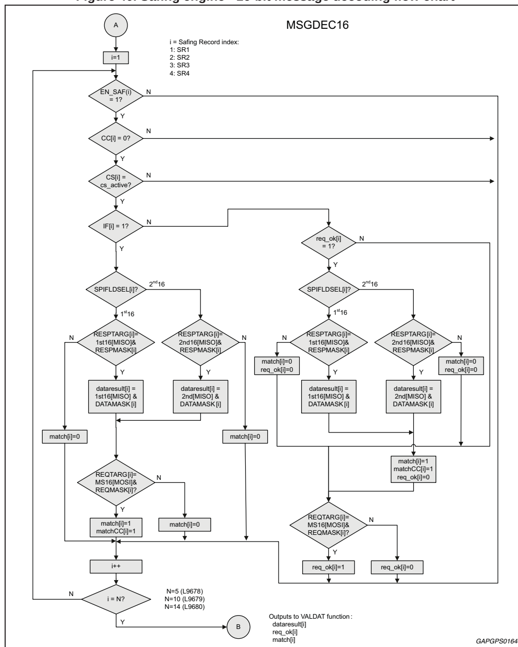
Figure 40. Safing engine - 16-bit message decoding flow chart
