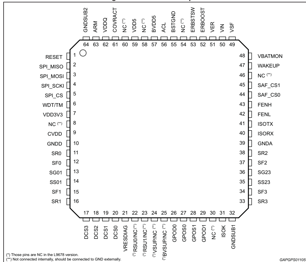
Figure 1. Pin-out description
