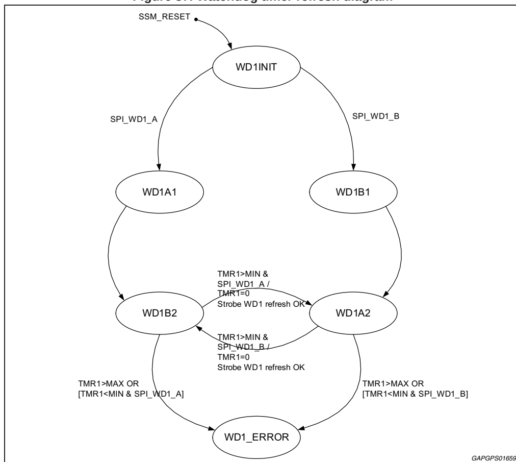
Figure 37. Watchdog timer refresh diagram
